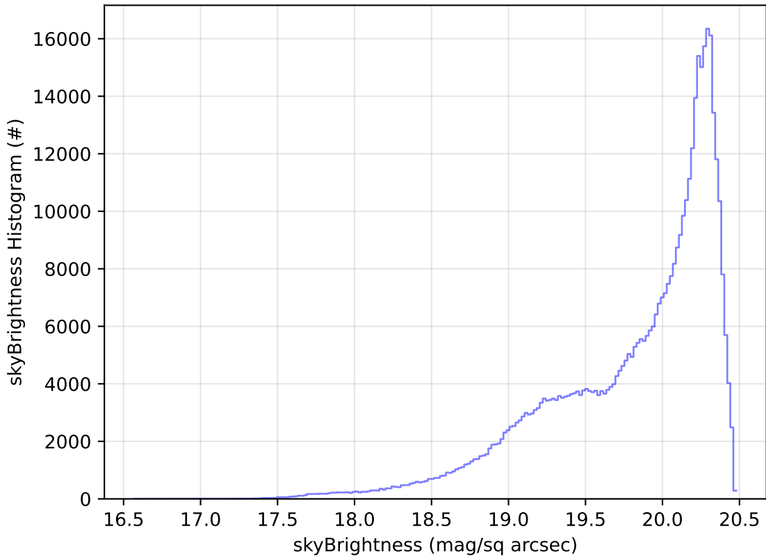
too_elab_r128_d3_ugrizy_v3.4_10yrs WFD i band: skyBrightness Histogram
