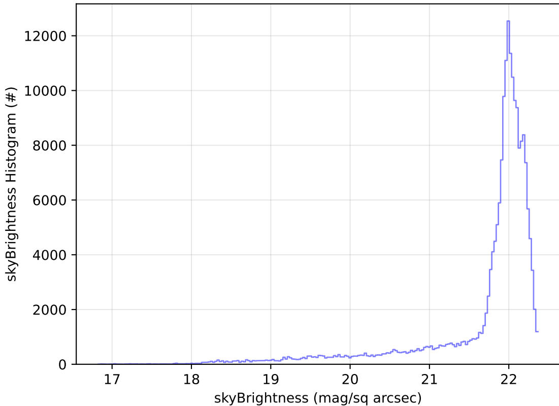
too_elab_r128_d3_ugrizy_v3.4_10yrs WFD g band: skyBrightness Histogram
