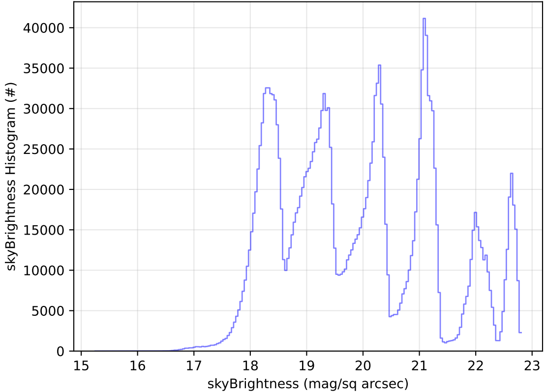
too_elab_r128_d3_ugrizy_v3.4_10yrs WFD all bands: skyBrightness Histogram
