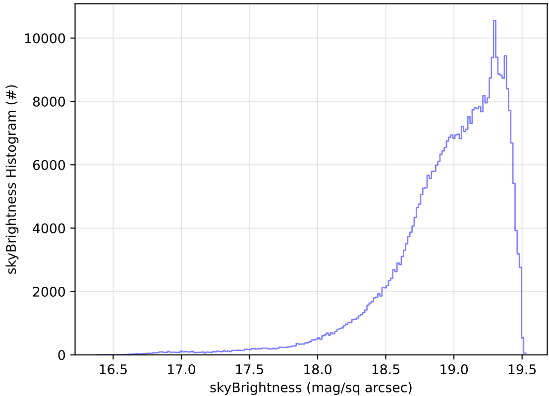
too_elab_r128_d3_ugrizy_v3.4_10yrs All sky z band: skyBrightness Histogram
