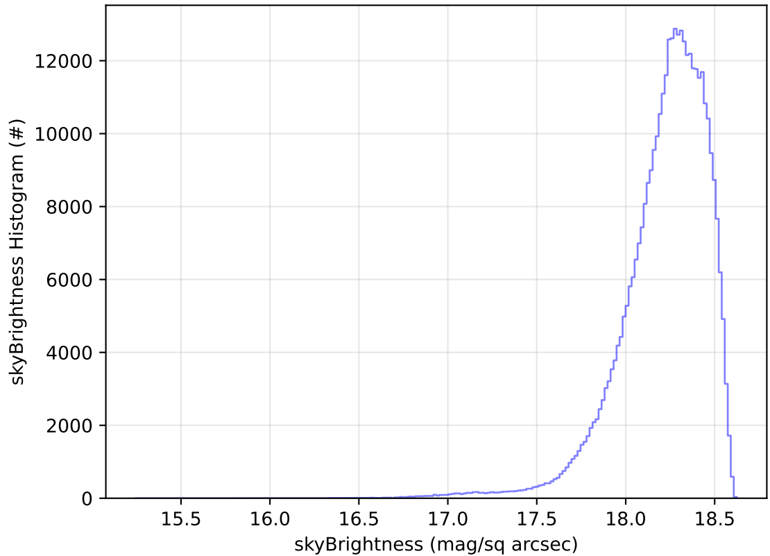
too_elab_r128_d3_ugrizy_v3.4_10yrs All sky y band: skyBrightness Histogram
