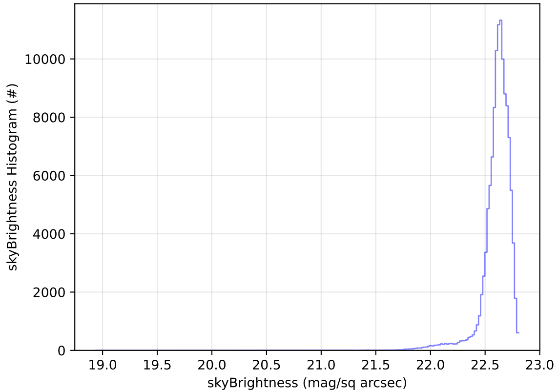
too_elab_r128_d3_ugrizy_v3.4_10yrs All sky u band: skyBrightness Histogram
