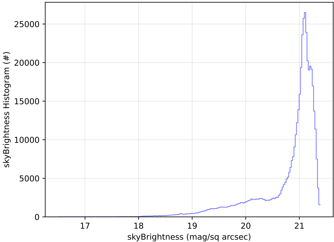
too_elab_r128_d3_ugrizy_v3.4_10yrs All sky r band: skyBrightness Histogram
