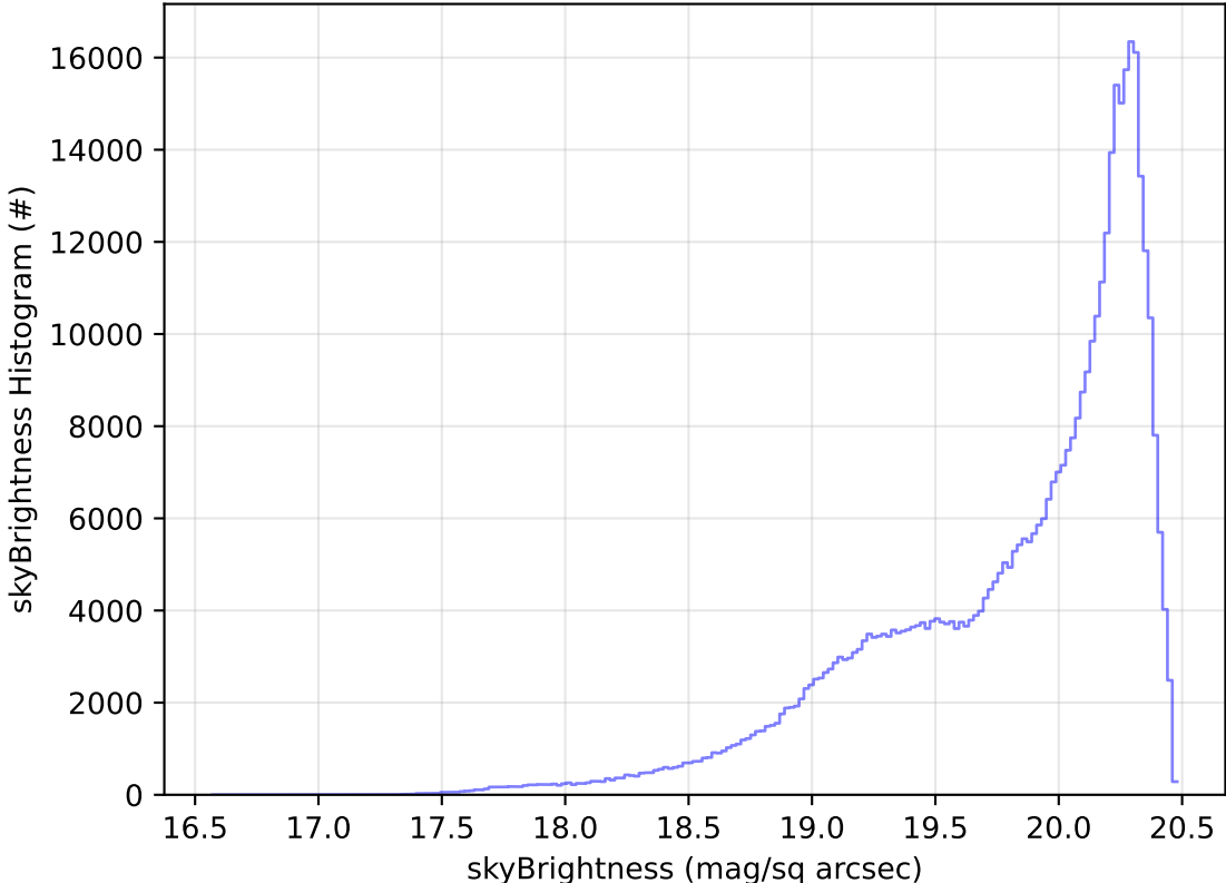
too_elab_r128_d3_ugrizy_v3.4_10yrs All sky i band: skyBrightness Histogram
