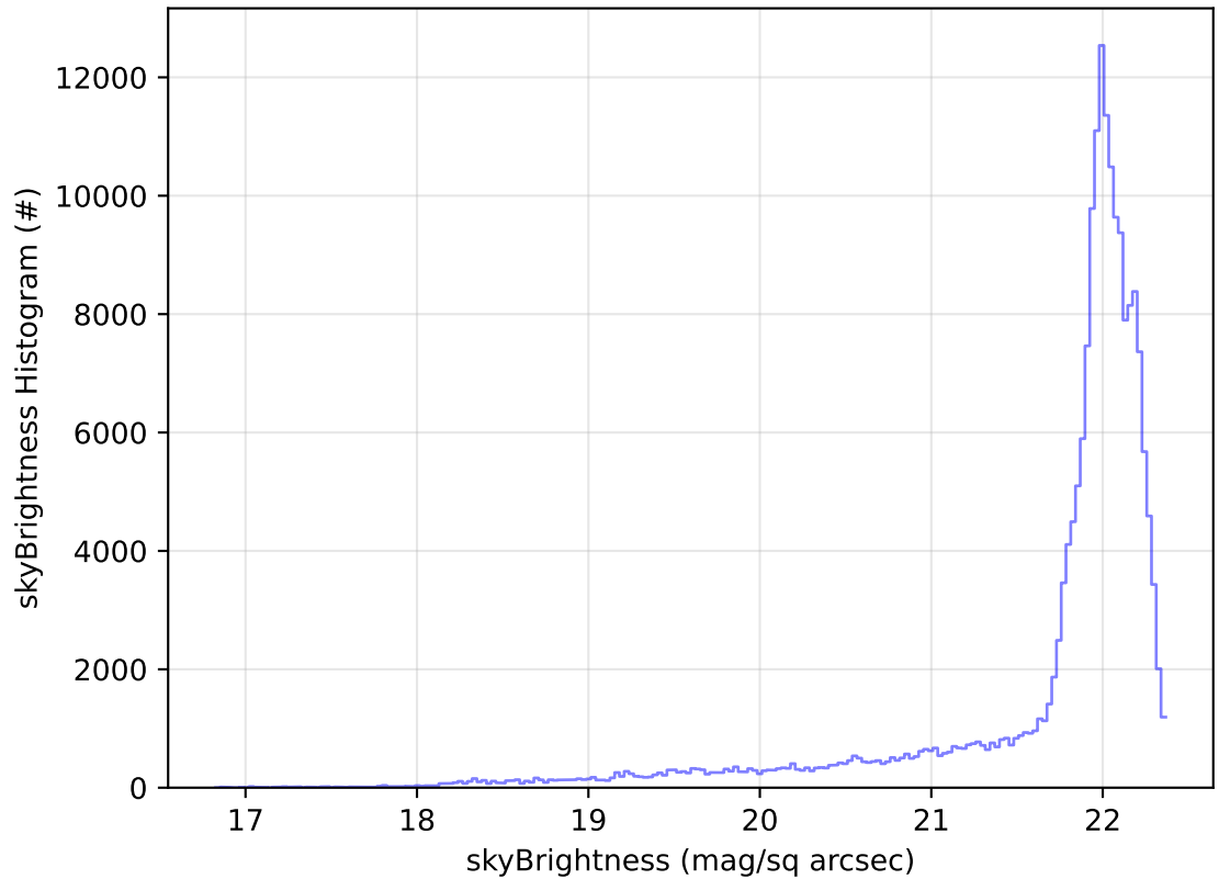
too_elab_r128_d3_ugrizy_v3.4_10yrs All sky g band: skyBrightness Histogram
