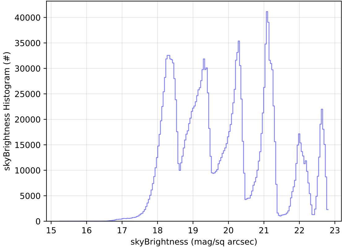
too_elab_r128_d3_ugrizy_v3.4_10yrs All sky all bands: skyBrightness Histogram
