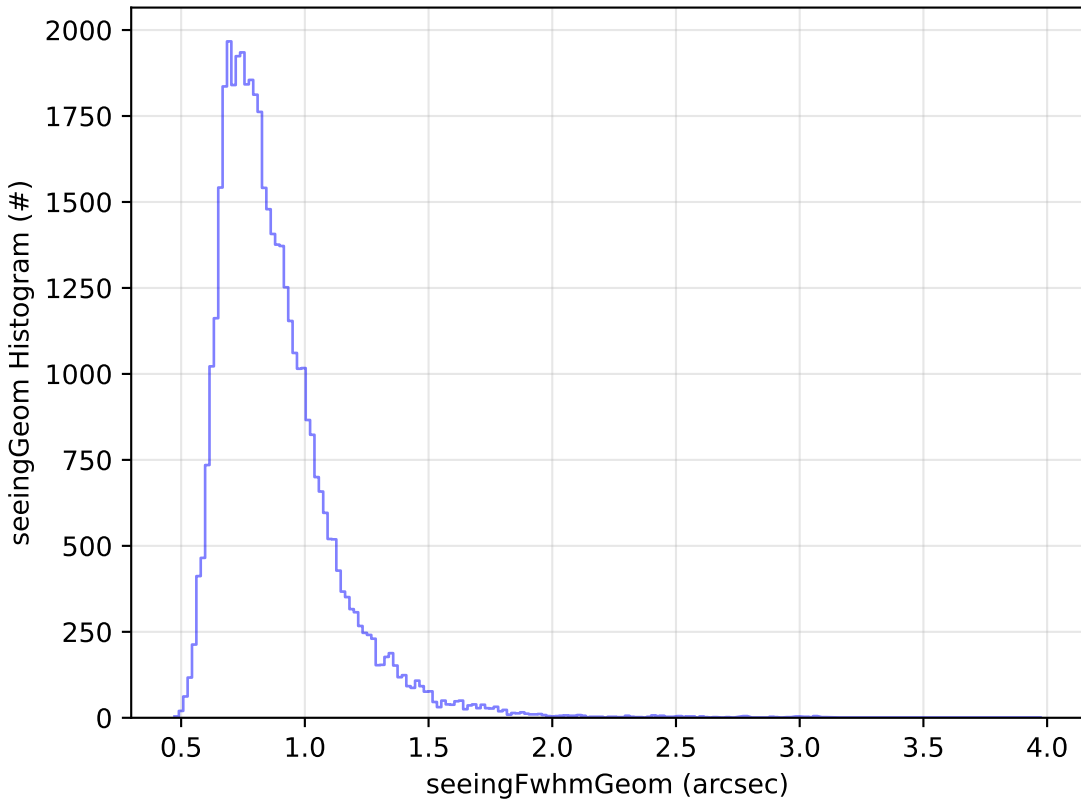
too_elab_r128_d3_ugrizy_v3.4_10yrs Yr 1 z band: seeingGeom Histogram
