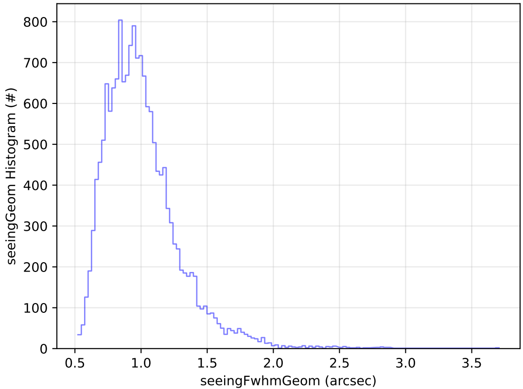
too_elab_r128_d3_ugrizy_v3.4_10yrs Yr 1 u band: seeingGeom Histogram
