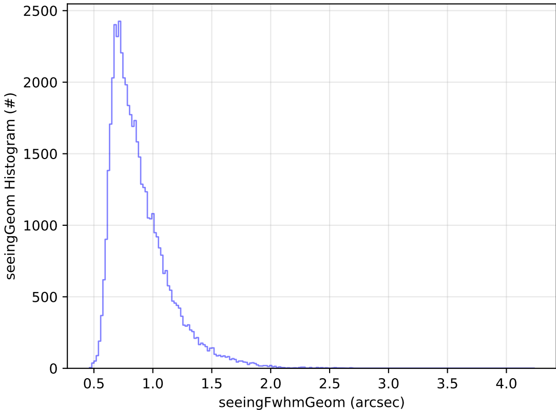
too_elab_r128_d3_ugrizy_v3.4_10yrs Yr 1 r band: seeingGeom Histogram
