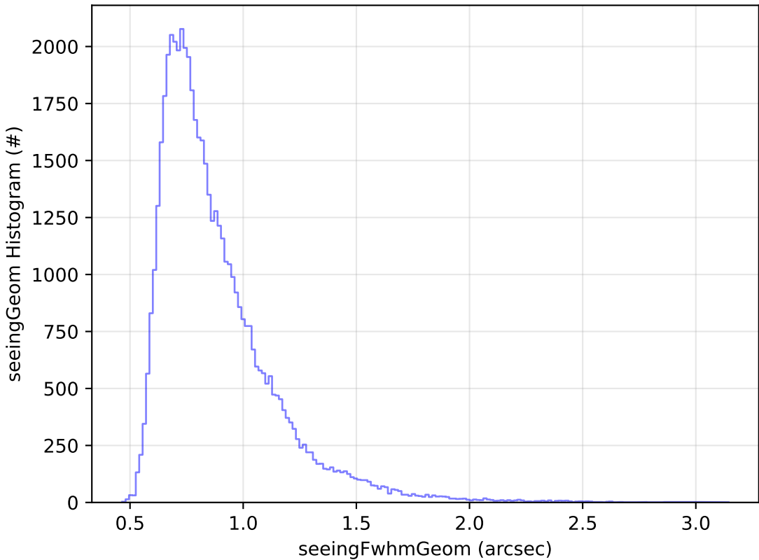
too_elab_r128_d3_ugrizy_v3.4_10yrs Yr 1 i band: seeingGeom Histogram
