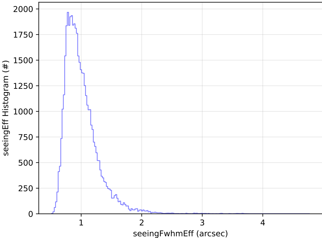
too_elab_r128_d3_ugrizy_v3.4_10yrs Yr 1 z band: seeingEff Histogram
