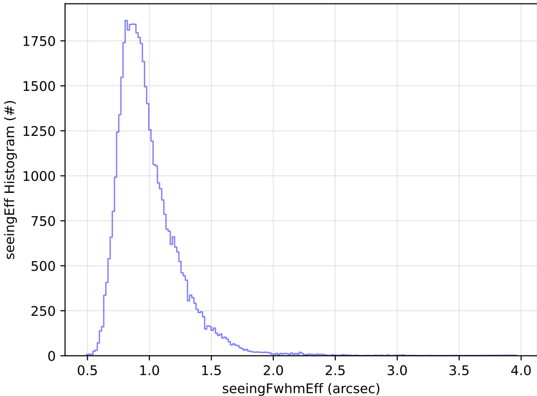
too_elab_r128_d3_ugrizy_v3.4_10yrs Yr 1 y band: seeingEff Histogram
