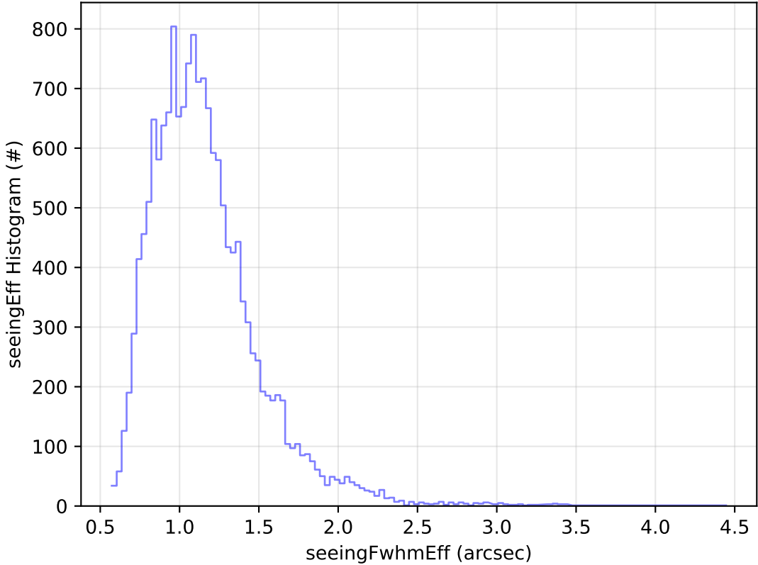
too_elab_r128_d3_ugrizy_v3.4_10yrs Yr 1 u band: seeingEff Histogram
