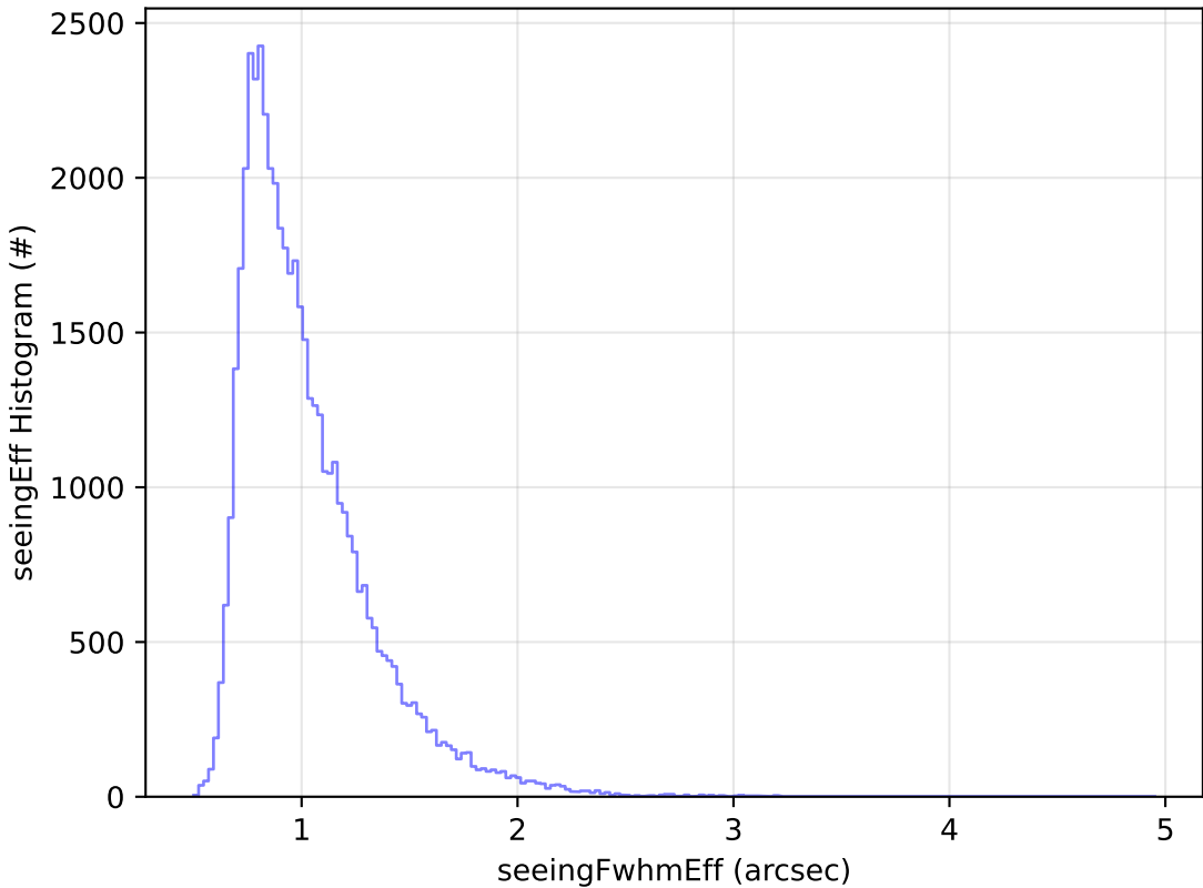
too_elab_r128_d3_ugrizy_v3.4_10yrs Yr 1 r band: seeingEff Histogram
