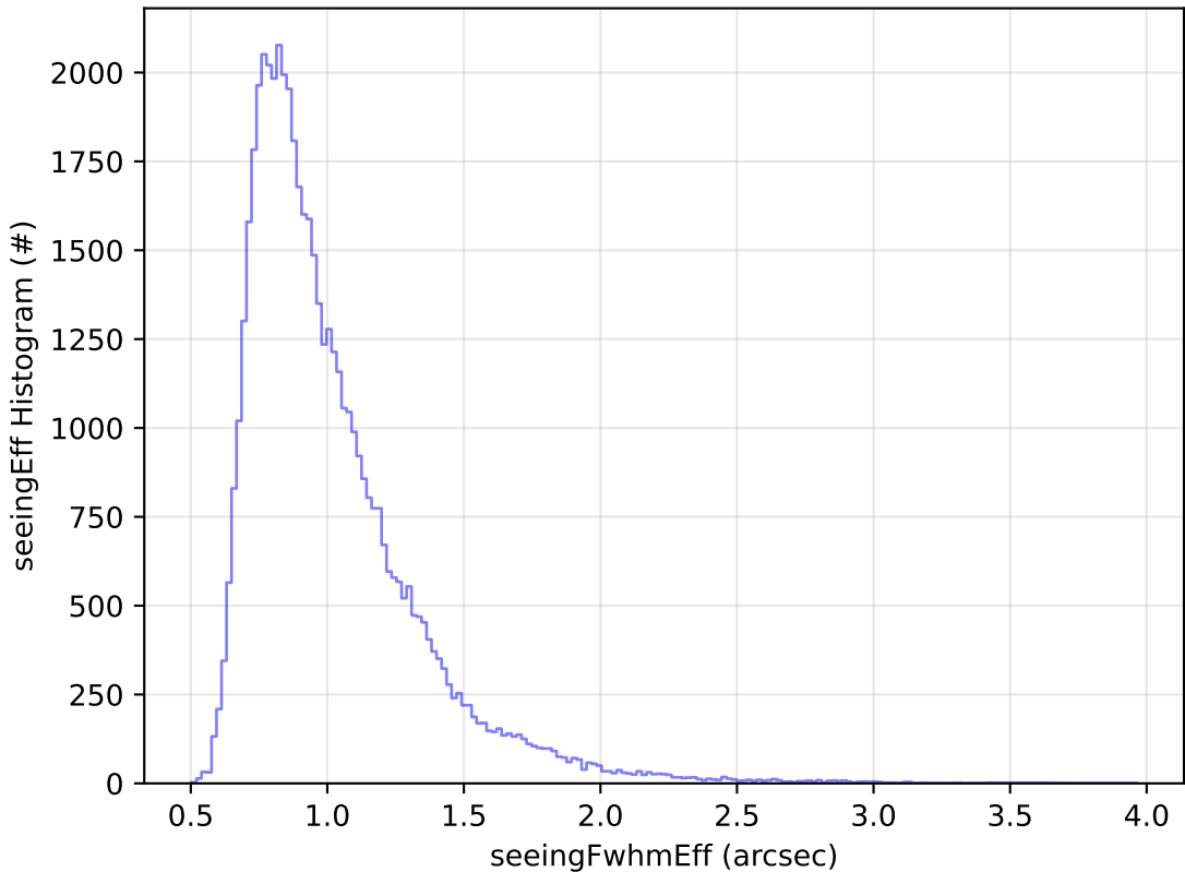
too_elab_r128_d3_ugrizy_v3.4_10yrs Yr 1 i band: seeingEff Histogram
