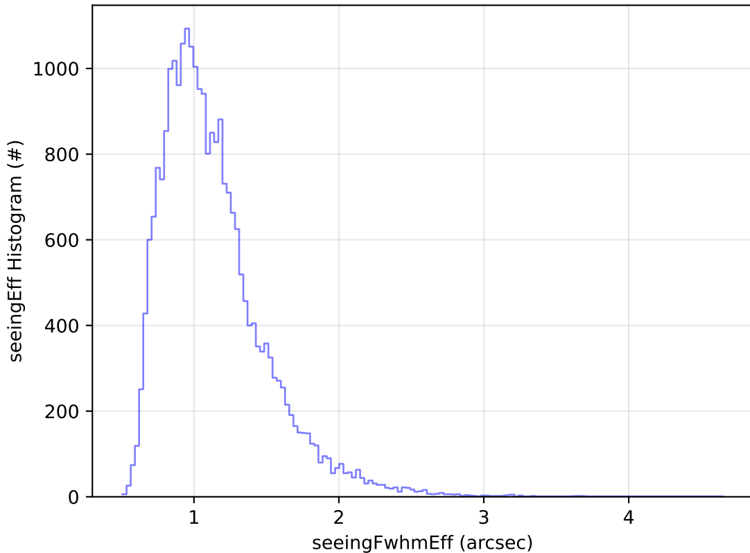
too_elab_r128_d3_ugrizy_v3.4_10yrs Yr 1 g band: seeingEff Histogram
