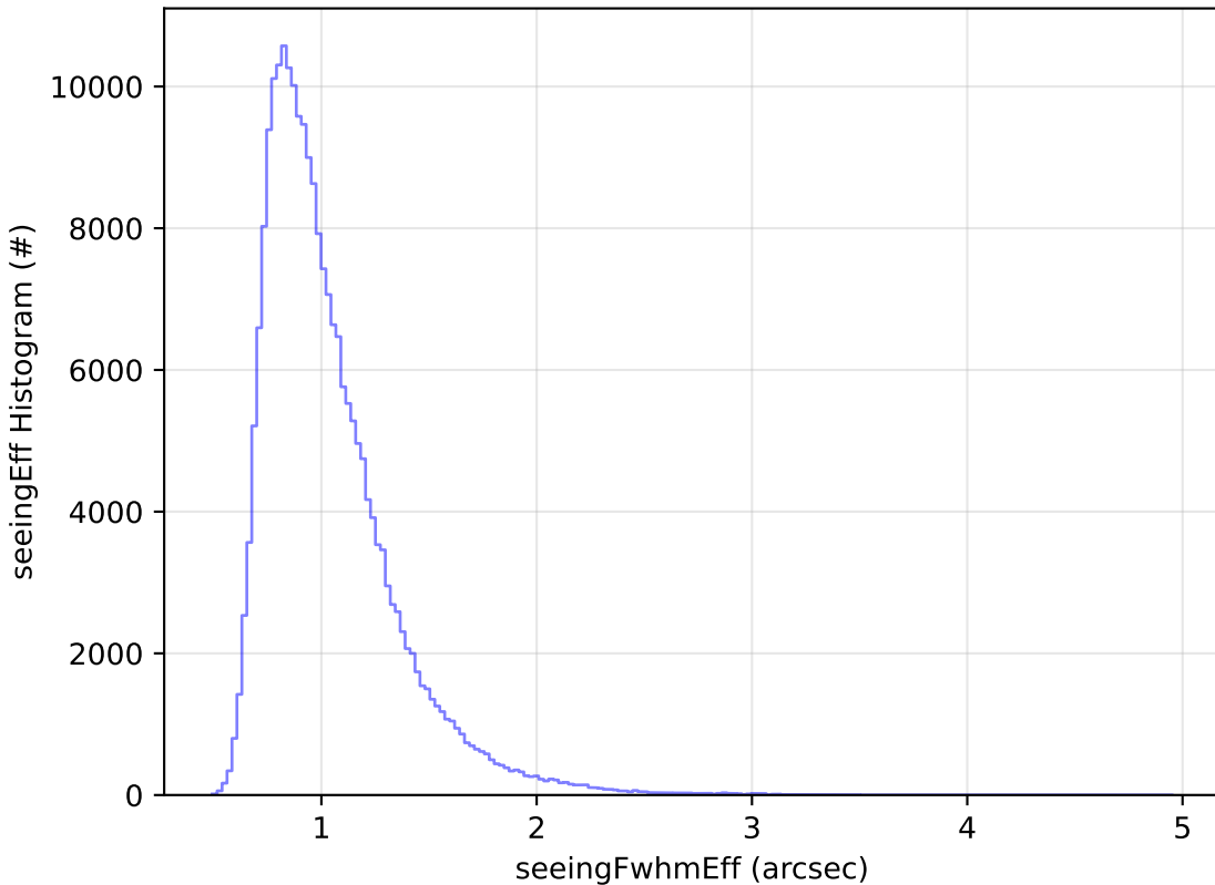
too_elab_r128_d3_ugrizy_v3.4_10yrs Yr 1 all bands: seeingEff Histogram
