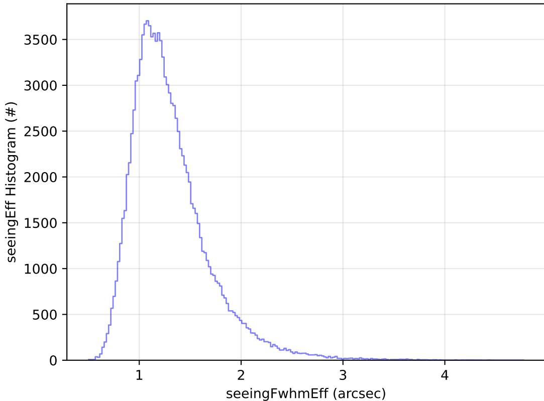
too_elab_r128_d3_ugrizy_v3.4_10yrs WFD u band: seeingEff Histogram
