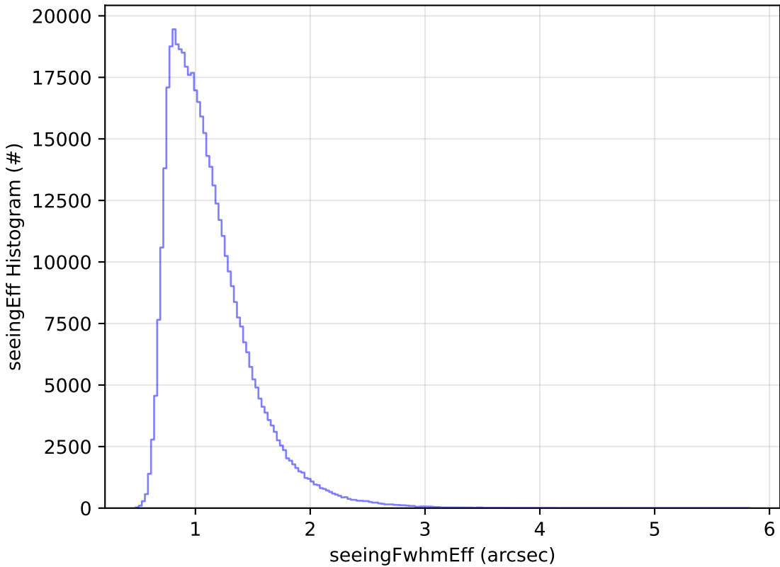
too_elab_r128_d3_ugrizy_v3.4_10yrs WFD r band: seeingEff Histogram
