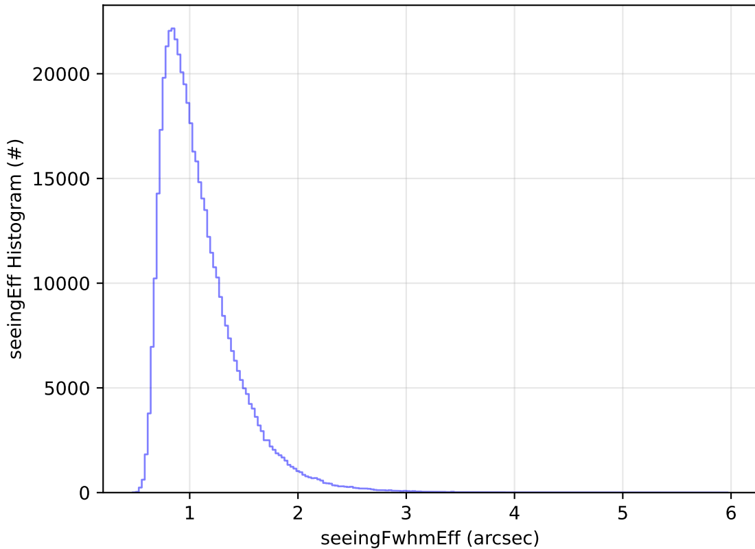
too_elab_r128_d3_ugrizy_v3.4_10yrs WFD i band: seeingEff Histogram
