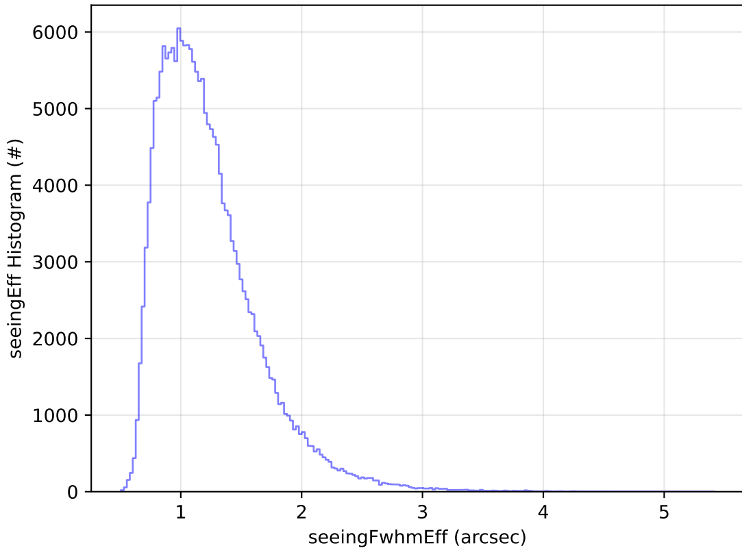
too_elab_r128_d3_ugrizy_v3.4_10yrs WFD g band: seeingEff Histogram
