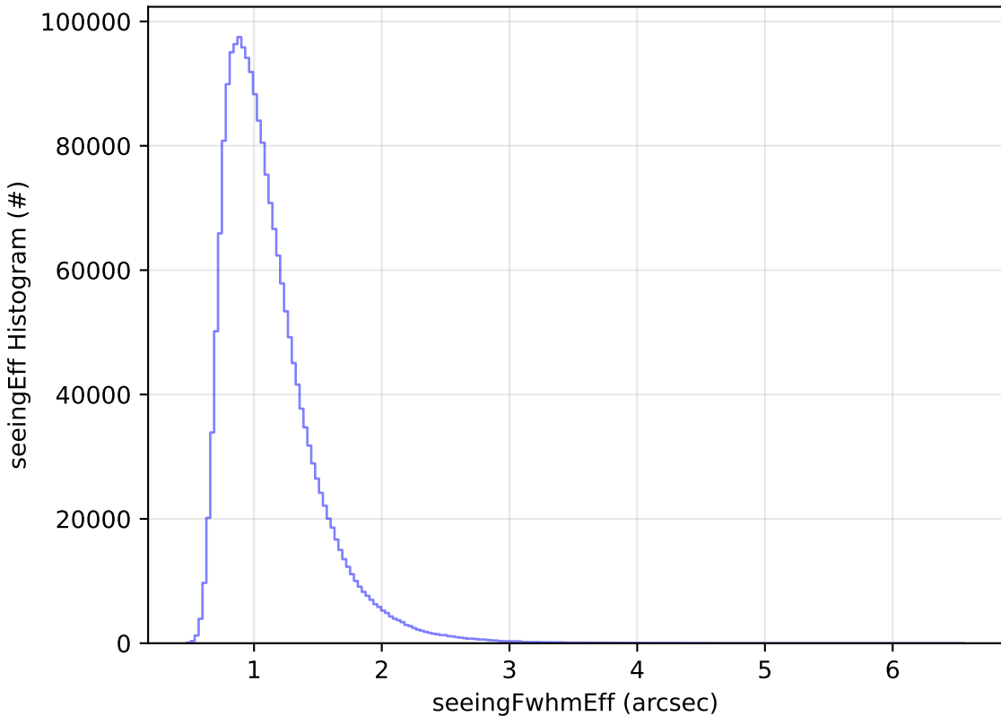
too_elab_r128_d3_ugrizy_v3.4_10yrs WFD all bands: seeingEff Histogram
