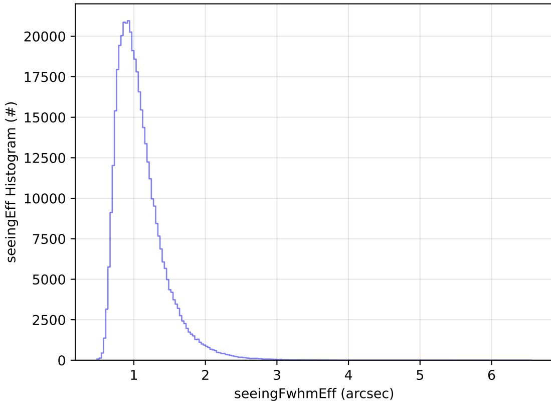
too_elab_r128_d3_ugrizy_v3.4_10yrs All sky z band: seeingEff Histogram
