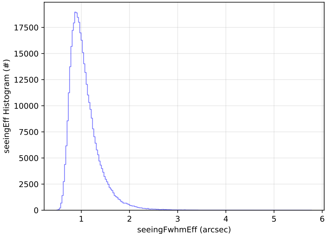
too_elab_r128_d3_ugrizy_v3.4_10yrs All sky y band: seeingEff Histogram
