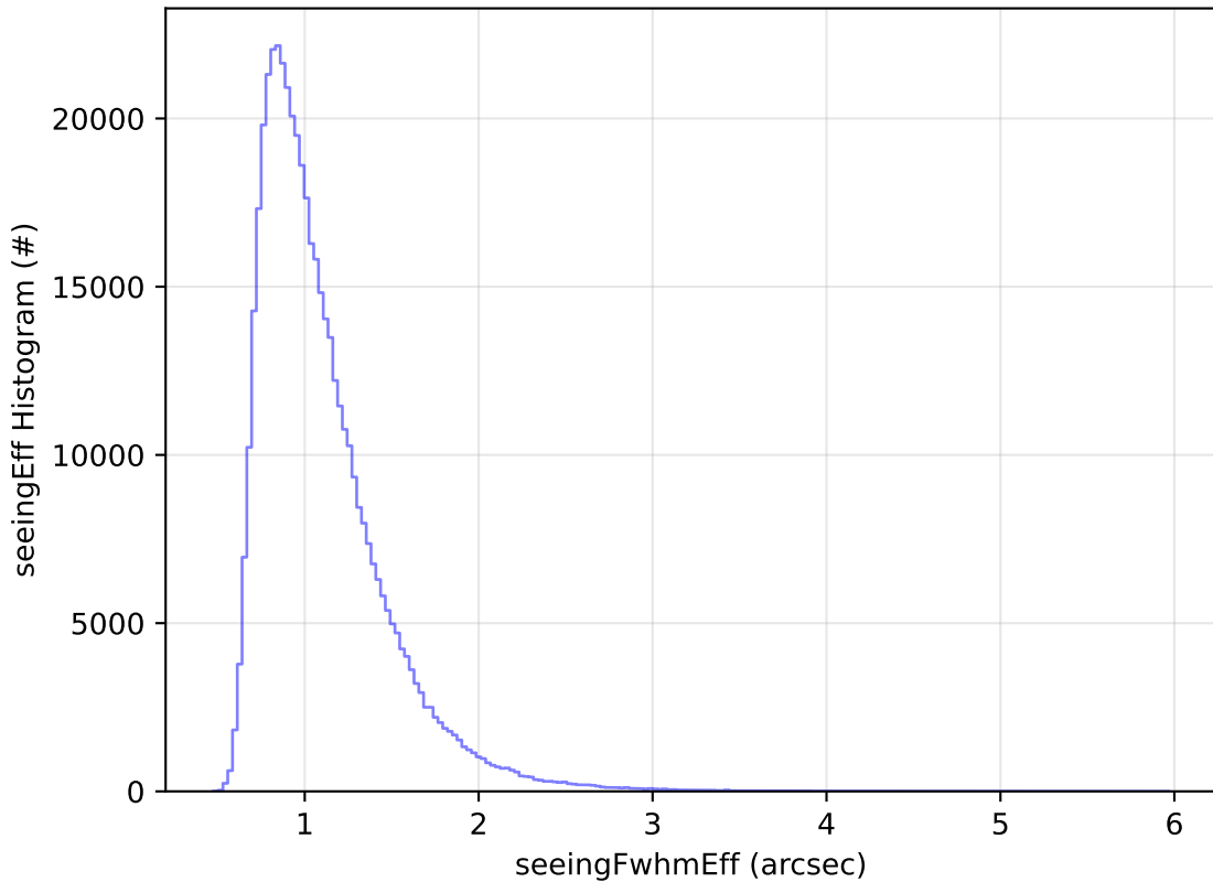
too_elab_r128_d3_ugrizy_v3.4_10yrs All sky i band: seeingEff Histogram
