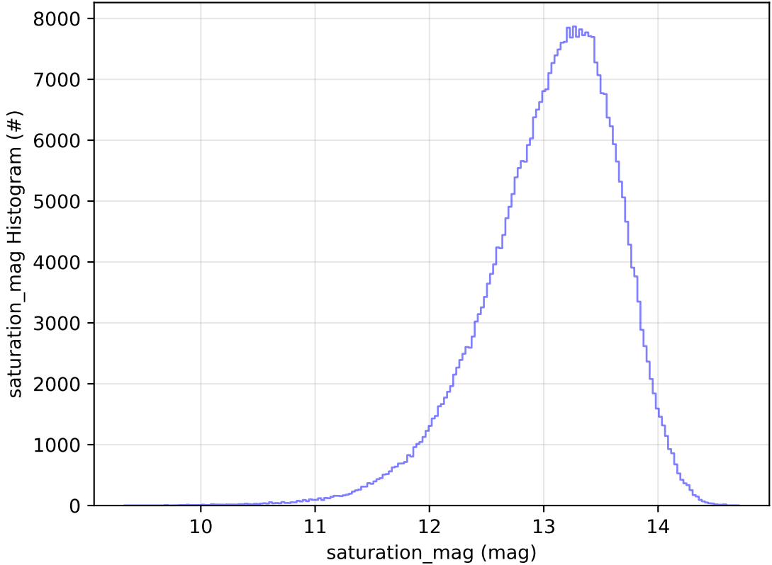
too_elab_r128_d3_ugrizy_v3.4_10yrs WFD y band: saturation_mag Histogram
