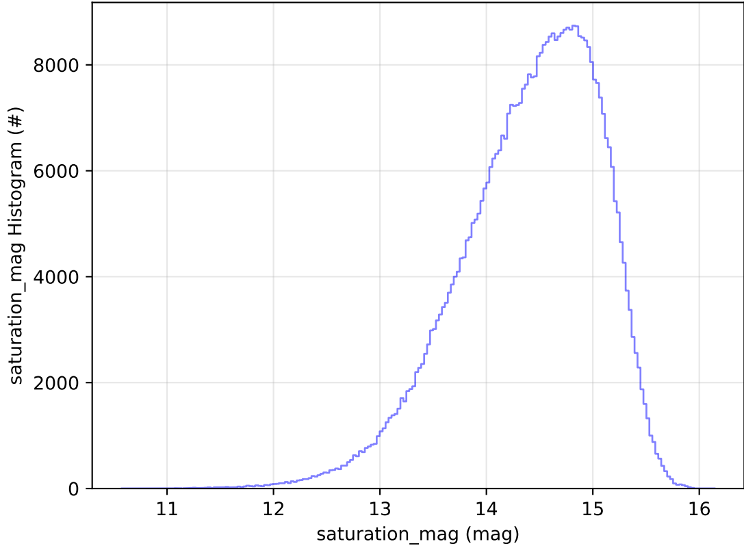
too_elab_r128_d3_ugrizy_v3.4_10yrs WFD i band: saturation_mag Histogram
