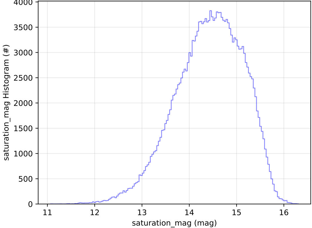
too_elab_r128_d3_ugrizy_v3.4_10yrs WFD g band: saturation_mag Histogram
