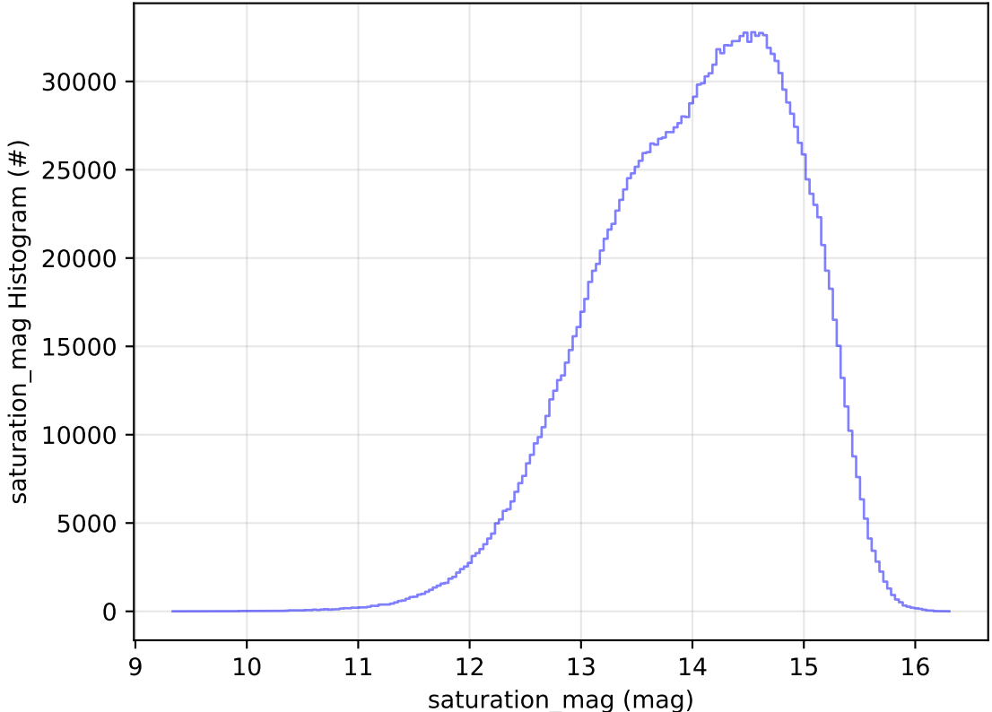
too_elab_r128_d3_ugrizy_v3.4_10yrs WFD all bands: saturation_mag Histogram
