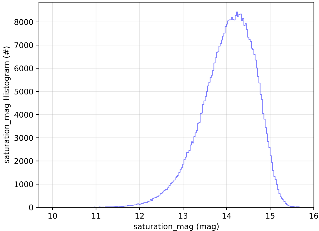
too_elab_r128_d3_ugrizy_v3.4_10yrs All sky z band: saturation_mag Histogram
