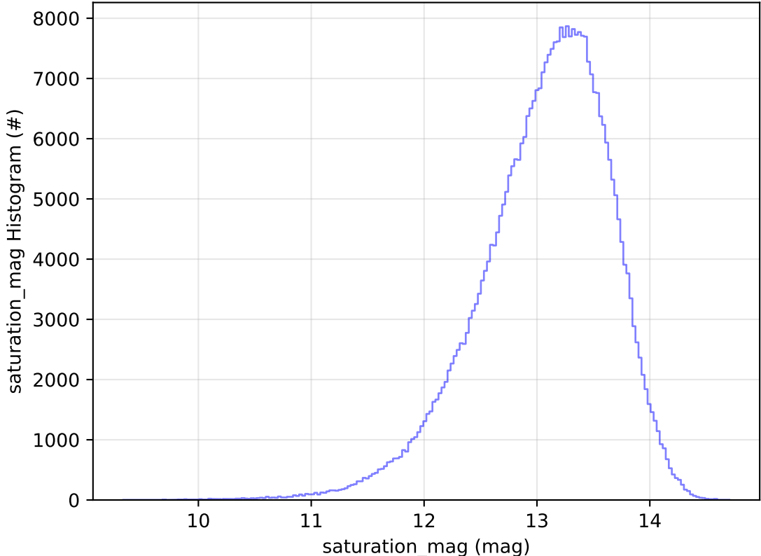
too_elab_r128_d3_ugrizy_v3.4_10yrs All sky y band: saturation_mag Histogram
