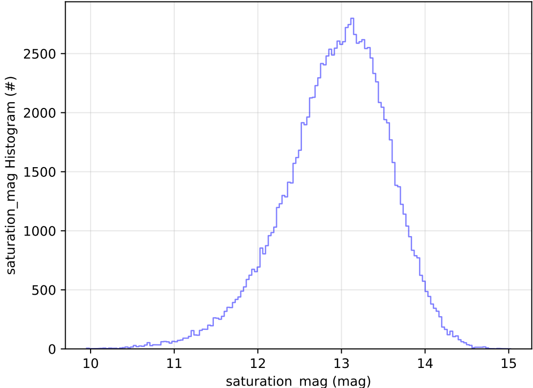
too_elab_r128_d3_ugrizy_v3.4_10yrs All sky u band: saturation_mag Histogram
