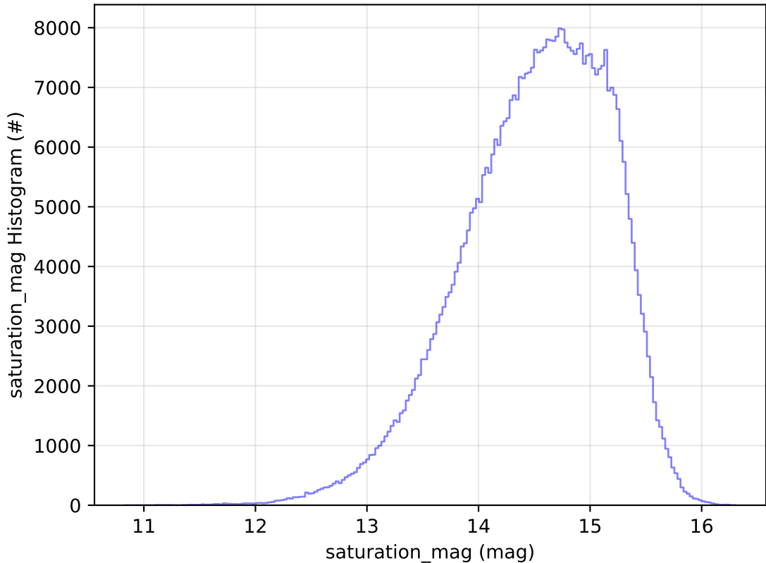
too_elab_r128_d3_ugrizy_v3.4_10yrs All sky r band: saturation_mag Histogram
