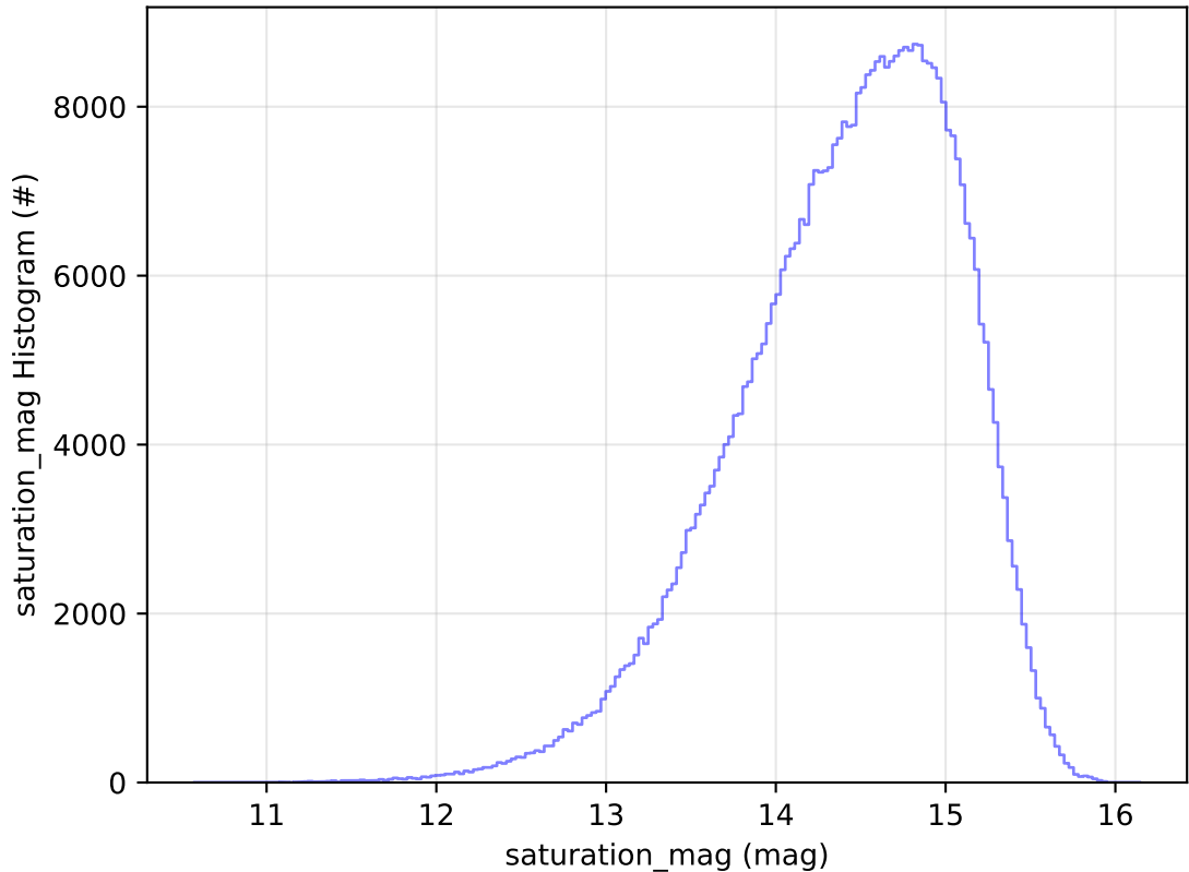
too_elab_r128_d3_ugrizy_v3.4_10yrs All sky i band: saturation_mag Histogram
