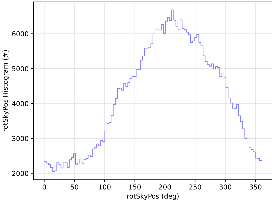
too_elab_r128_d3_ugrizy_v3.4_10yrs WFD z band: rotSkyPos Histogram
