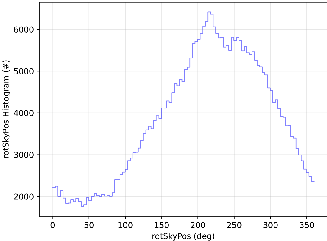
too_elab_r128_d3_ugrizy_v3.4_10yrs WFD y band: rotSkyPos Histogram
