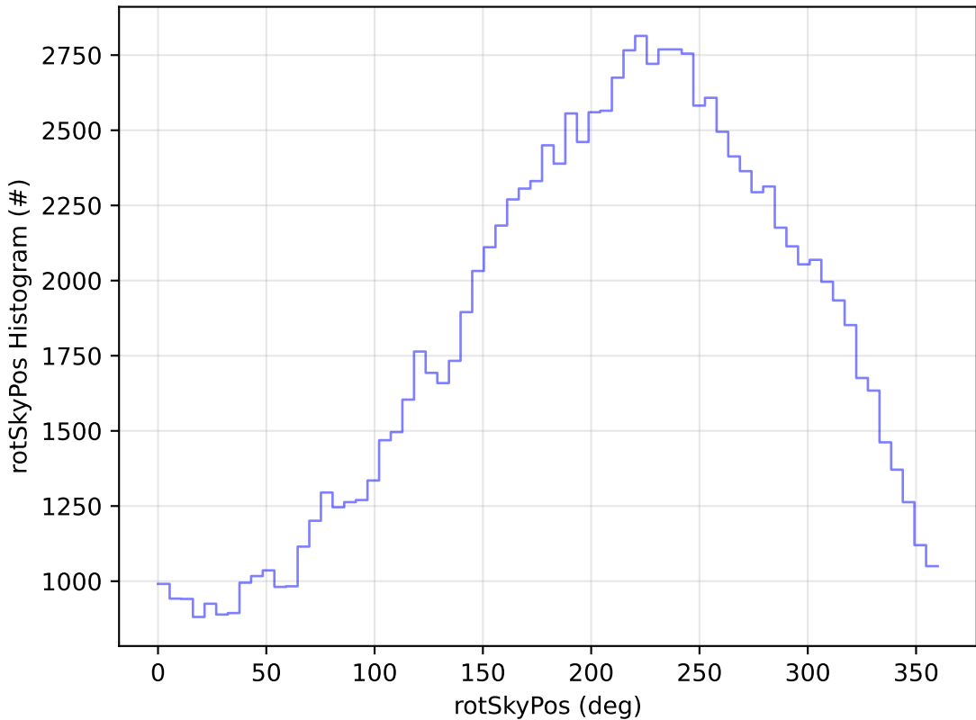
too_elab_r128_d3_ugrizy_v3.4_10yrs WFD u band: rotSkyPos Histogram
