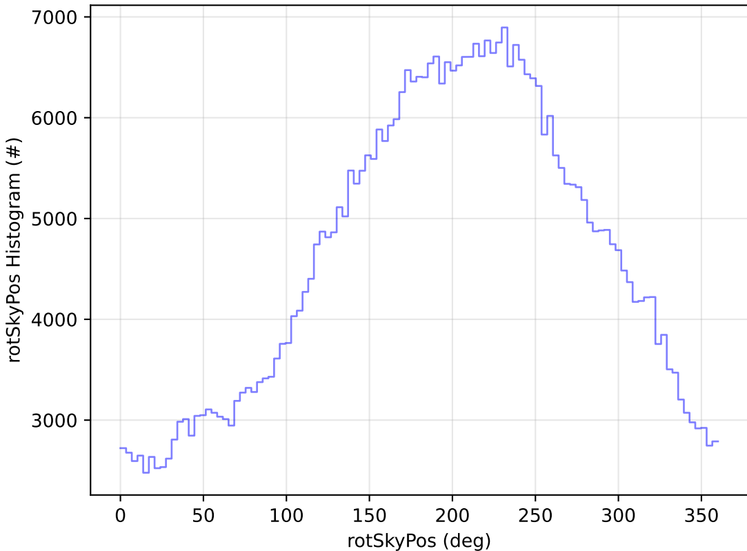
too_elab_r128_d3_ugrizy_v3.4_10yrs WFD r band: rotSkyPos Histogram
