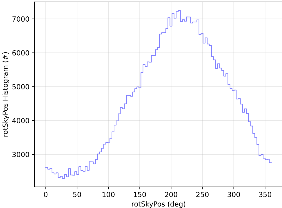
too_elab_r128_d3_ugrizy_v3.4_10yrs WFD i band: rotSkyPos Histogram
