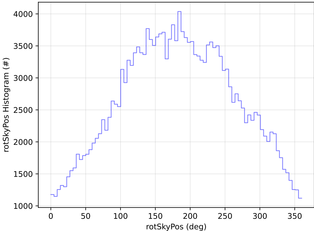
too_elab_r128_d3_ugrizy_v3.4_10yrs WFD g band: rotSkyPos Histogram
