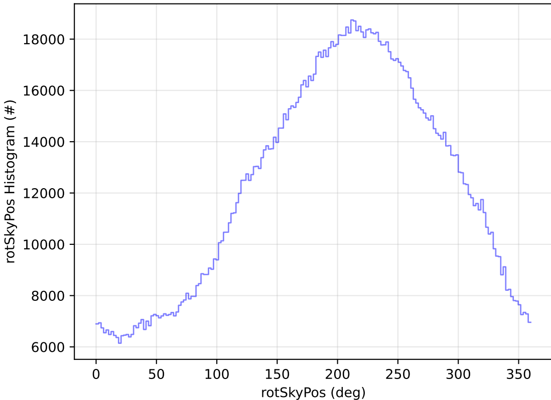
too_elab_r128_d3_ugrizy_v3.4_10yrs WFD all bands: rotSkyPos Histogram
