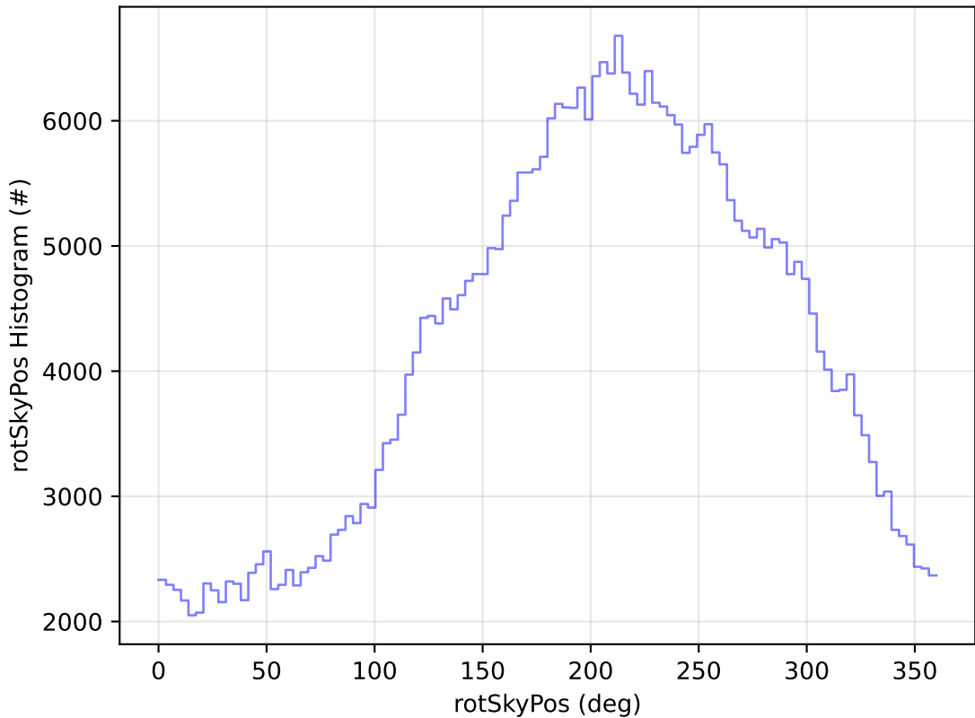
too_elab_r128_d3_ugrizy_v3.4_10yrs All sky z band: rotSkyPos Histogram
