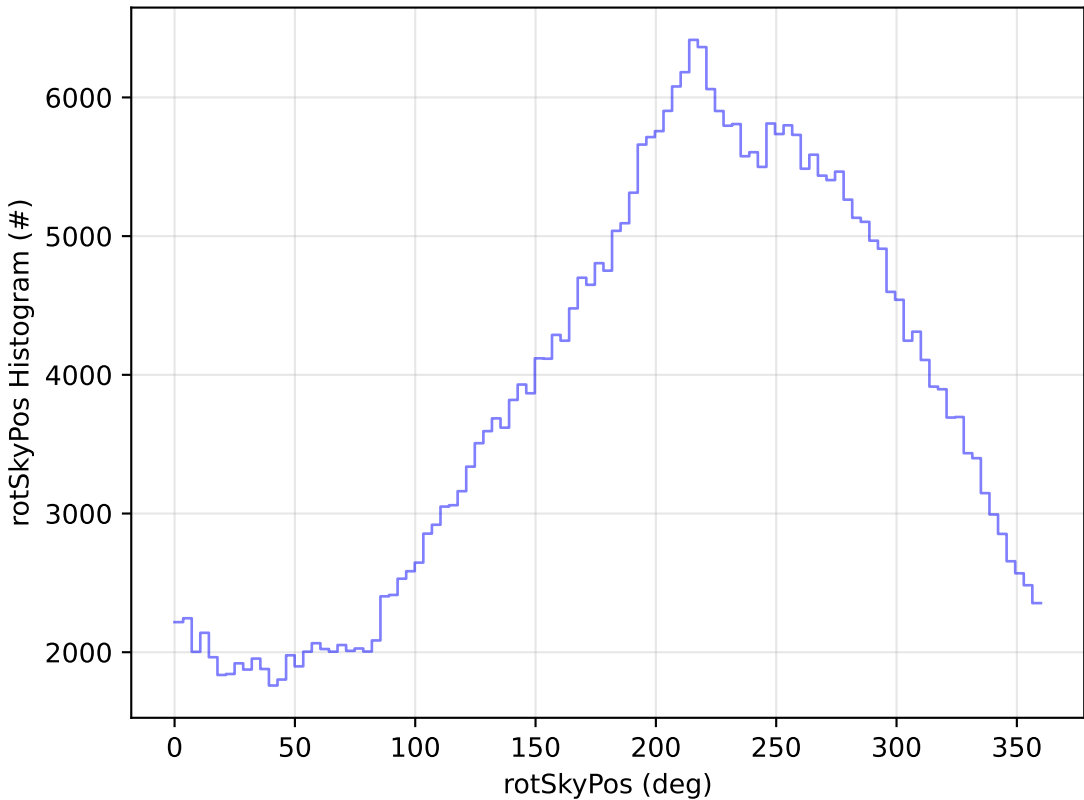
too_elab_r128_d3_ugrizy_v3.4_10yrs All sky y band: rotSkyPos Histogram
