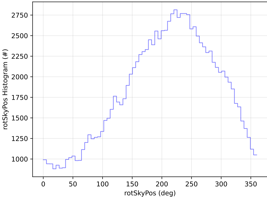
too_elab_r128_d3_ugrizy_v3.4_10yrs All sky u band: rotSkyPos Histogram
