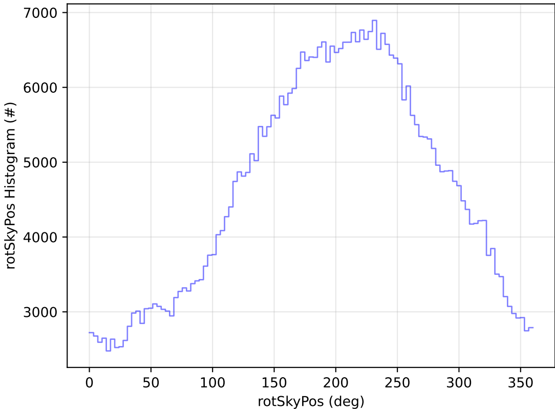
too_elab_r128_d3_ugrizy_v3.4_10yrs All sky r band: rotSkyPos Histogram
