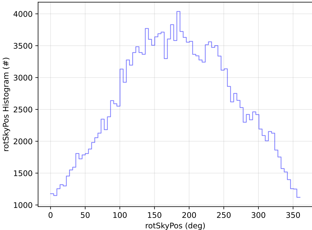
too_elab_r128_d3_ugrizy_v3.4_10yrs All sky g band: rotSkyPos Histogram
